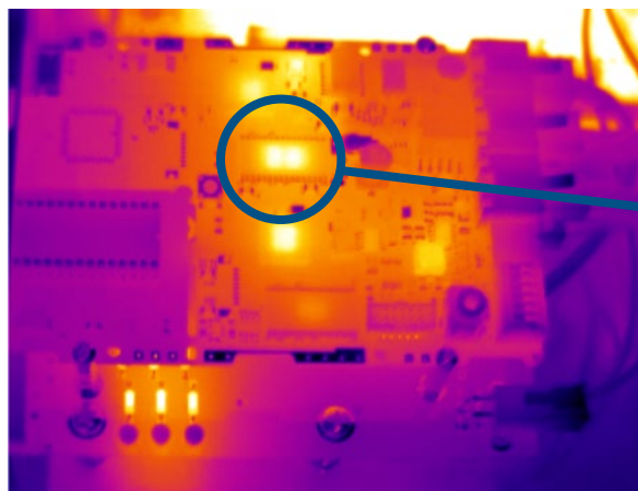
Figure 4. Thermal image of a PCA
