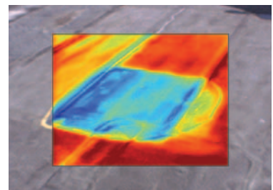
Roofing: Detect water-saturated insulation in flat-roof systems to locate damaged portions of roofing structure.
