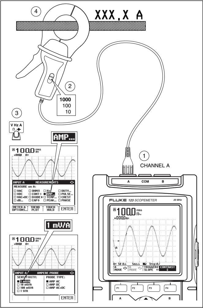
Figure 3. ScopeMeter Setups
