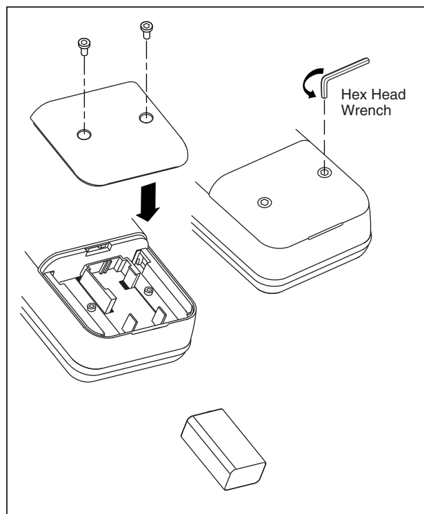
Figure 7. Battery Replacement
