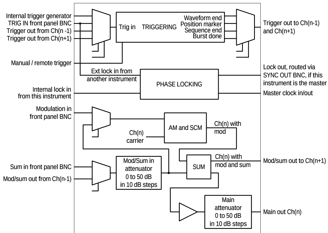
Figure F-1. Block Diagram: Single Channel
