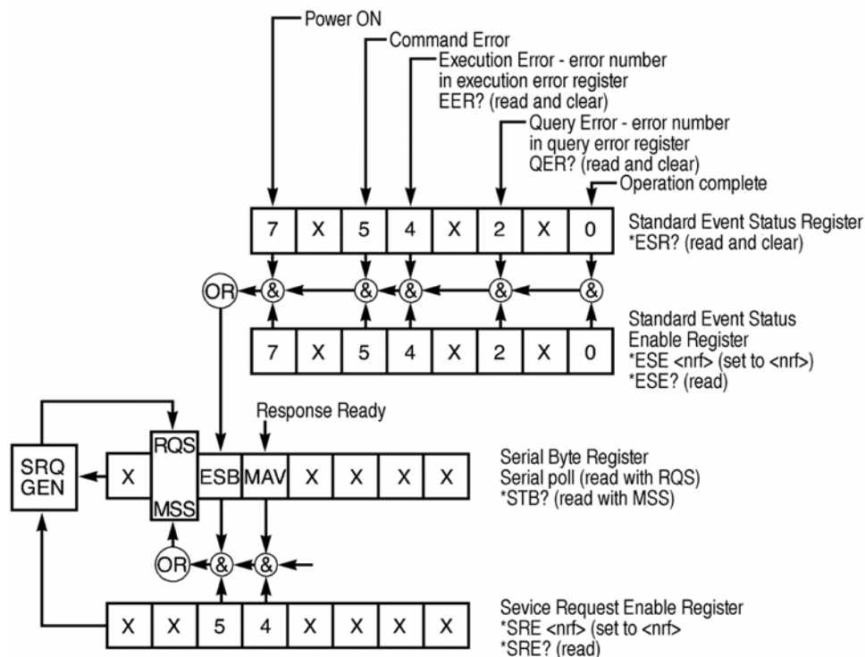
Figure 17-4. Status Model
